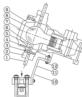
For Reflex Gauge A-A' VIEW
