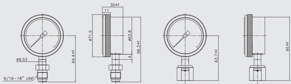
Swivel male
