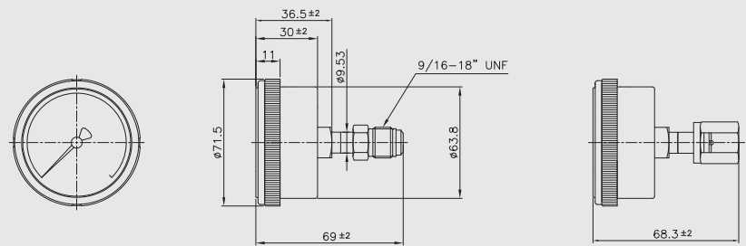
Swivel male
